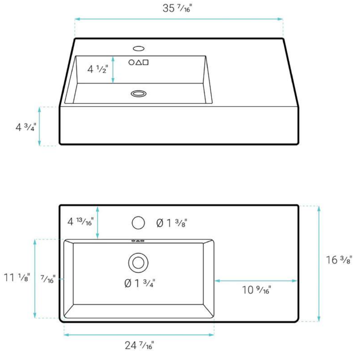
Wall-Mount Sink
