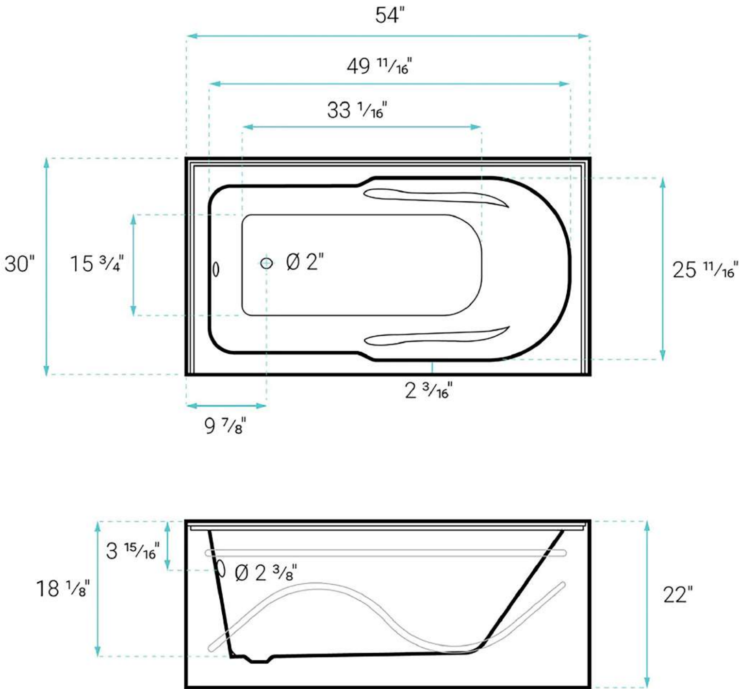
Alcove Bathtub
